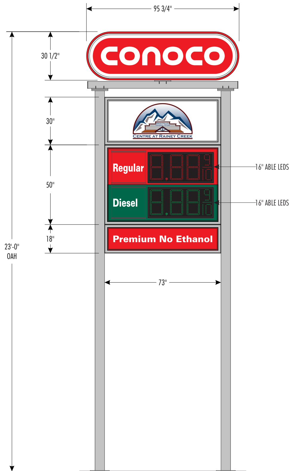
FRONT VIEW
